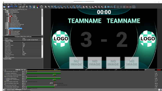
Template Editor
